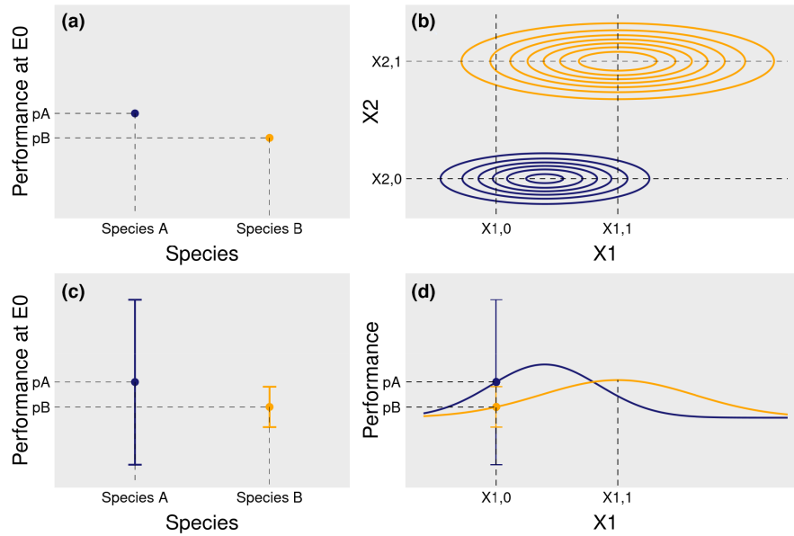
FIGURE 3 Reinterpreting observed intraspecific variability (IV): from niche widening to niche projection into a high-dimensional environment. In (a), within a given environment E0 defined along an environmental axis X1 ( E0 = E(X1,0) ), conspecific individuals are identical and have the same performance pA and pB, for species A (blue) and species B (orange). Species A outcompetes species B in E0. Actual measured differences among conspecific individuals, shown in (c), can be interpreted in different ways. First, as conspecific individuals exhibit contrasting attributes in E0, they become more different. This can result in some heterospecific individuals having similar performances: IV would make species less different. Alternatively, IV measured in E0 results from the variation of unobserved environmental variables ( E0 = E(X1,0, X2) ; (b)). Contrasting performances among conspecific individuals in E0 do not result from intrinsic differences among them but from differences in the local environment they experience and that was poorly characterized, that is, the number of observed dimensions is lower than the actual number of environmental dimensions. Similarly, although species niches present some overlap when projected on one dimension (d), they do not overlap in the two-dimensional space (b). Moreover, while species A outcompetes species B on average when X1 = X1,0 , the opposite occurs when X1 = X1,1 (d), leading to an inversion of species hierarchy between different environments. Similarly, while species A outcompetes species B in E(X1,0, X2,0) , the opposite occurs in E(X1,0, X2,1) . Although only two dimensions are shown, species respond to many environmental variables varying in space and time, multiplying the possibilities of niche segregation and hierarchy inversions between species, offering room for species coexistence in a variable high-dimensional environment. The code used to generate this figure is available online.
